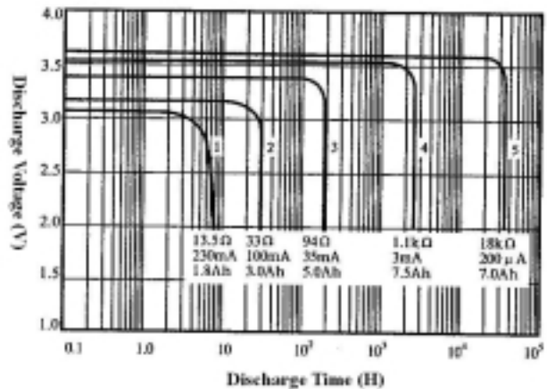
Discharge Characteristics at 25°C
