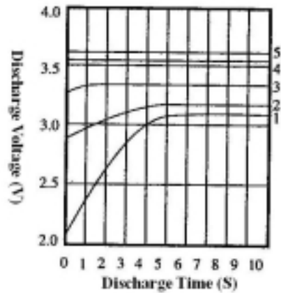
Activation Characteristics at 25°C
