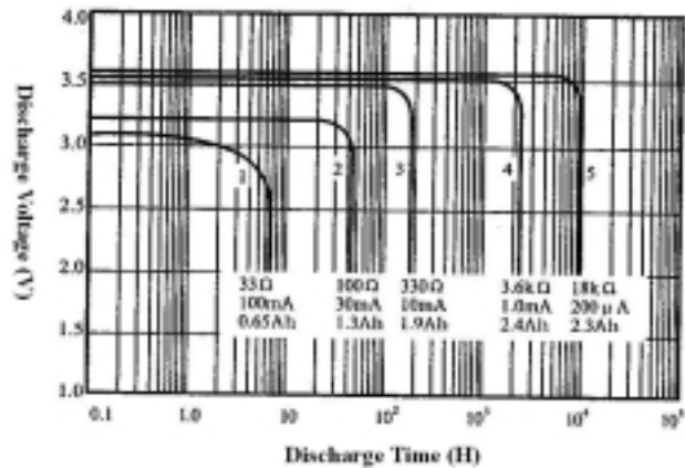
Discharge Characteristics at 25°C
