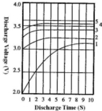
Activation Characteristics at 25°C
