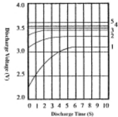
Activation Characteristics at 25°C
