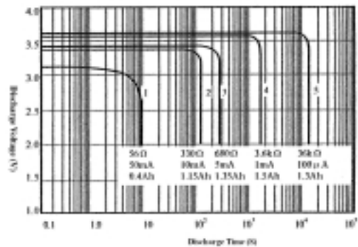
Discharge Characteristics at 25°C
