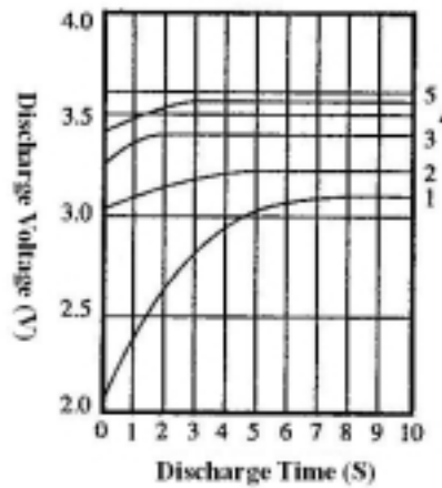
Activation Characteristics at 25°C
