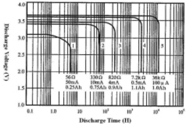
Discharge Characteristics at 25°C
