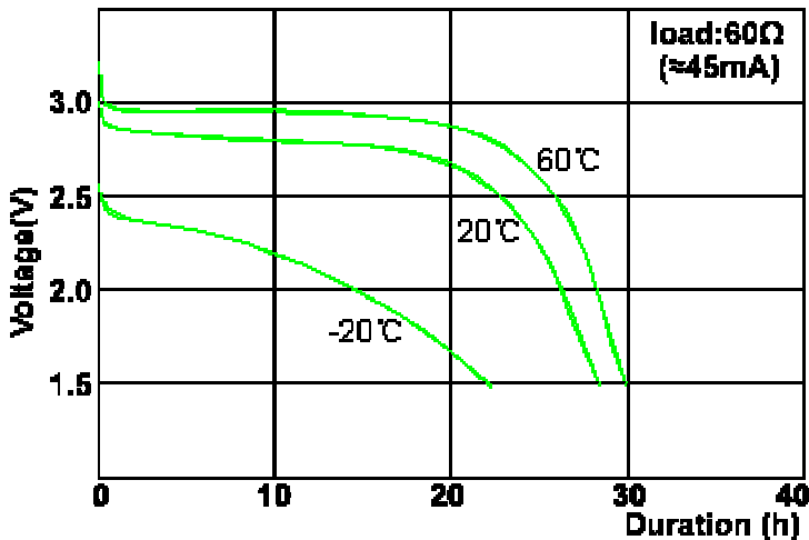
Temperature characteristics
