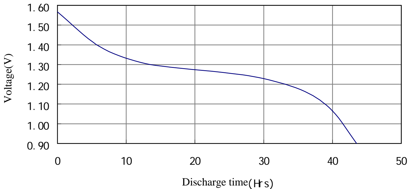
Typical Discharge Characteristics (20°C)
